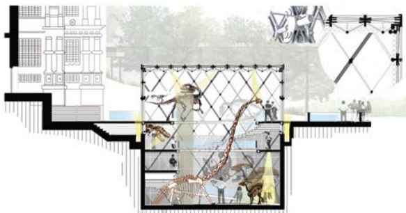
Section for the 'New Wollaton Hall Extension', completed as one of the Master's design projects (Distinction).
